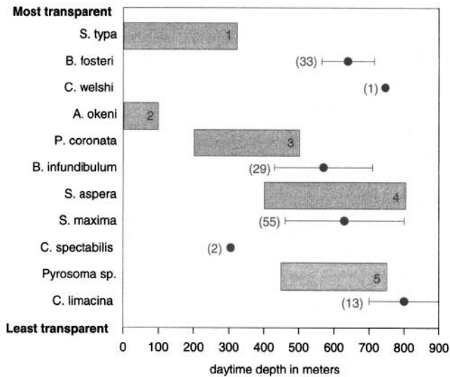
Figure 3. Transparency of species collected from Oceanographer Canyon in relation to depth of daytime distribution. Species are arranged from most transparent ( Sibogita typha ) to least transparent ( Clione limacina ). Transparency values (filled circles) for each species are means of measurements taken from animals collected on the same cruise; bars are standard deviation of the mean, with number of specimens given in parentheses. Daytime depth ranges (bars) are taken from the literature. The number within each bar gives the reference from which it was taken: 1 = Mayer (1910); 2 = Youngbluth (pers. comm.); 3 = Lalli and Gilmer (1989); 4 = Wiebe et al. (1979); 5 = Anderson et al. (1992).
